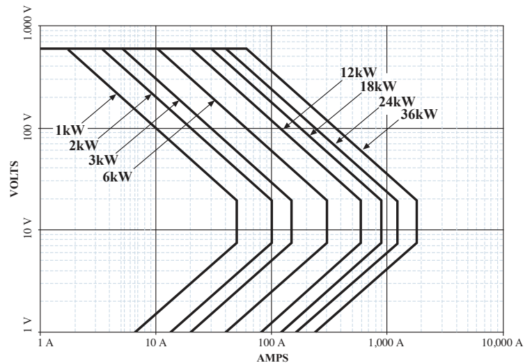
Constant power operating envelopes
